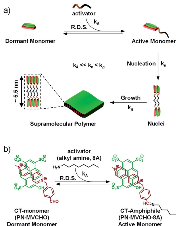
Scheme 1 (a) Schematic illustration of the chemical reaction (imine bond)-driven activation of a dormant monomer (charge-transfer (CT)-monomer) to an active monomer (CT-amphiphile) by an activator which further undergoes nucleation-growth into bilayer sheets. (b) Chemical structure and reaction for the activation of a CT-complex composed of a pyranine (PN) donor and methyl viologen benzaldehyde (MVCHO) acceptor to the CT-amphiphile by octyl amine (8A). k_A = rate of activation, k_n = rate of nucleation, k_g = rate of growth/elongation and R.D.S. = rate determining step.
