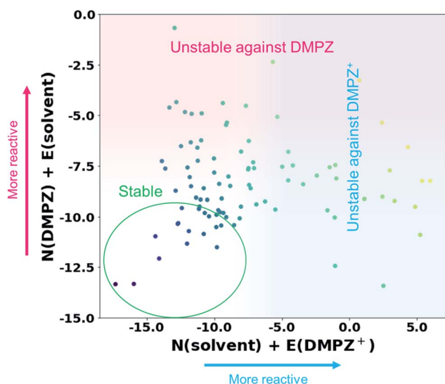
Fig. 3 Reactivity map showing N + E values, i.e. , \log_{10}(k_{\text{reaction}}) values, of 93 solvents against the electrophilic attack of DMPZ^+ and the nucleophilic attack of DMPZ .
