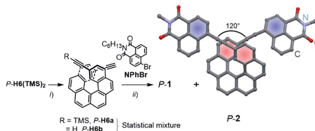
Scheme 1 Synthesis of enantiopure naphthalimide-helicene derivatives P-1 and P-2 . TMS: trimethylsilyl, C_6H_{13} : n -hexyl. Reaction conditions: (i) TBAF, CHCl_3 ; (ii) Pd(PPh_3)_4 , CuI, Et_3N /toluene, 50 °C, NPhBr , 85% ( P-1 ) and 90% ( P-2 ). X-ray crystal structure of P-2 (hexyl chains on the imide fragments have been omitted for clarity).
