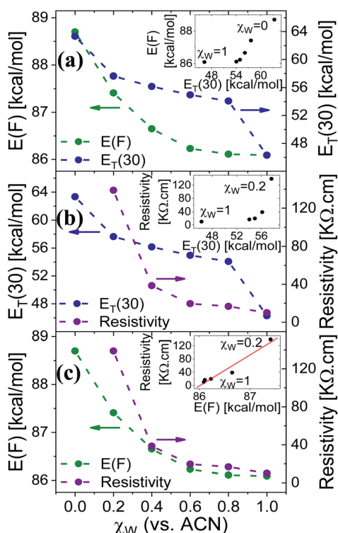
Fig. 4 The dependence of (a) E(F) and E_{T(30)} , (b) E_{T(30)} and resistivity, (c) E(F) and resistivity, as a function of the water fraction (within ACN), \chi_w , in the mat (for E(F) or resistivity) or in bulk solution (for E_{T(30)} ). The insets of (a and b) show the non-linear dependence of E(F) or resistivity vs. E_{T(30)} , and the one of (c) shows the linear dependence of the resistivity vs. E(F) .
