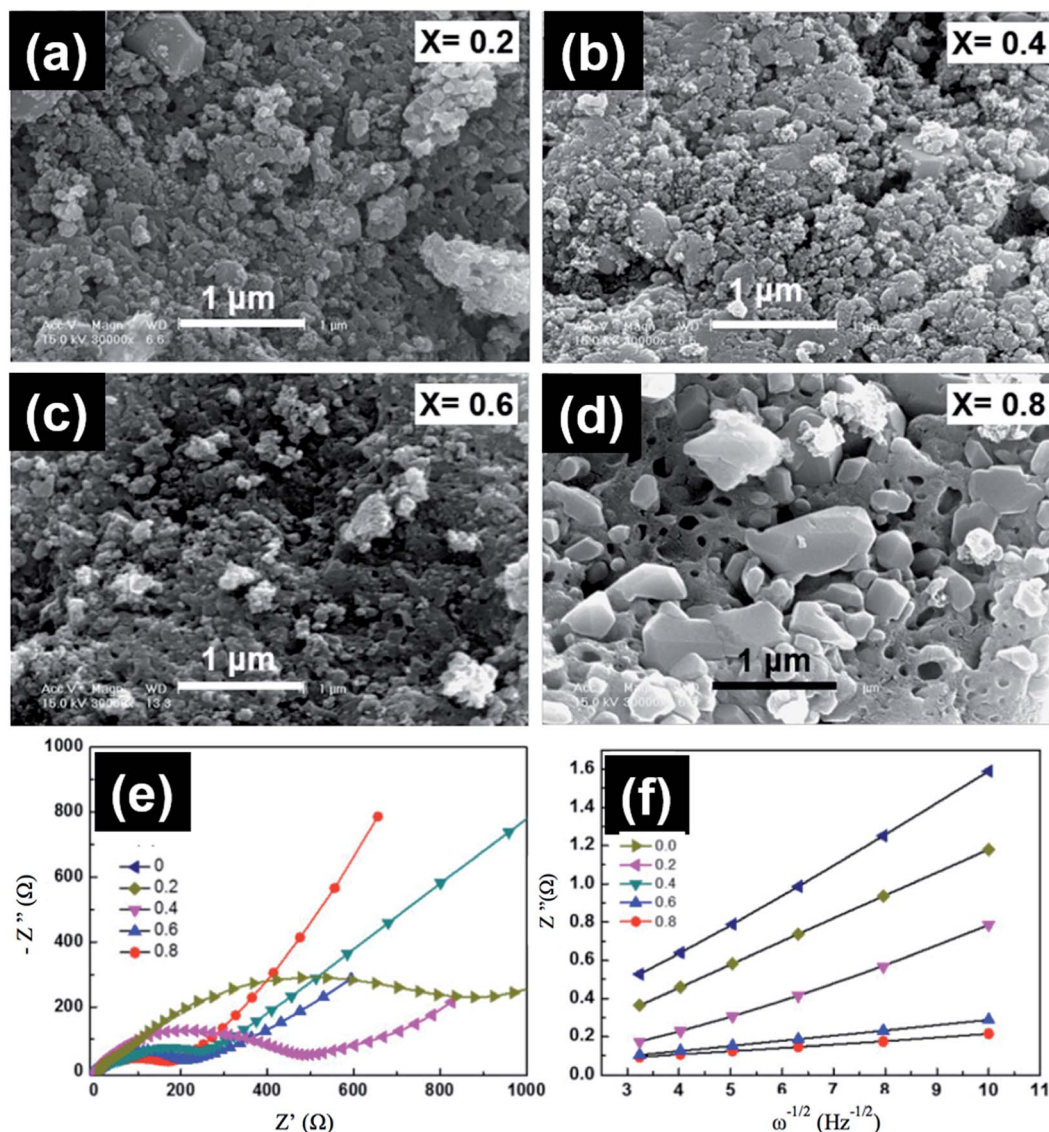
Fig. 13 (a–d) FESEM images, (e) impedance spectra, and (f) the relationship between Z'' and the square root of frequency ( \omega^{-1/2} ) in the low-frequency region for LiMn 1-x Fe x PO 4 at different compositions. 131
