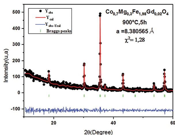
Fig. 3 Typical Rietveld-refined XRD pattern for the Co 0.7 Mg 0.3 Fe 1.98 Gd 0.02 O 4 sample.
