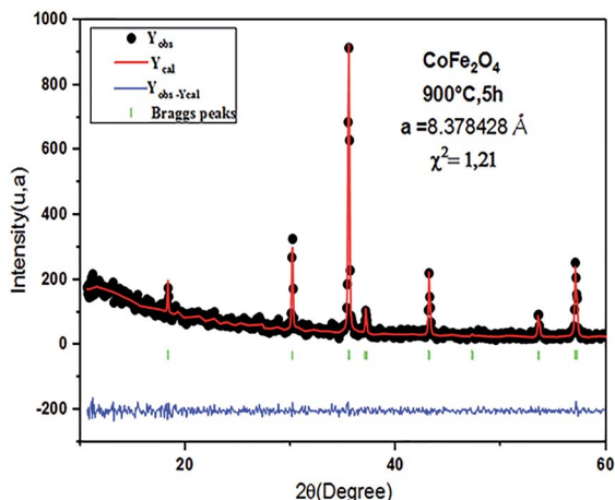
Fig. 2 Typical Rietveld-refined XRD pattern for the CoFe 2 O 4 sample.
