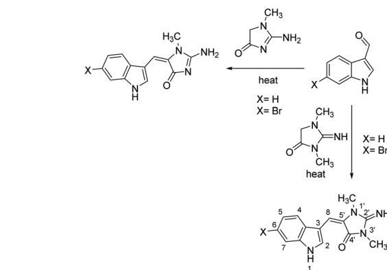
Scheme 29 First reported total synthesis of ( E )-aplysinopsin derivatives.
