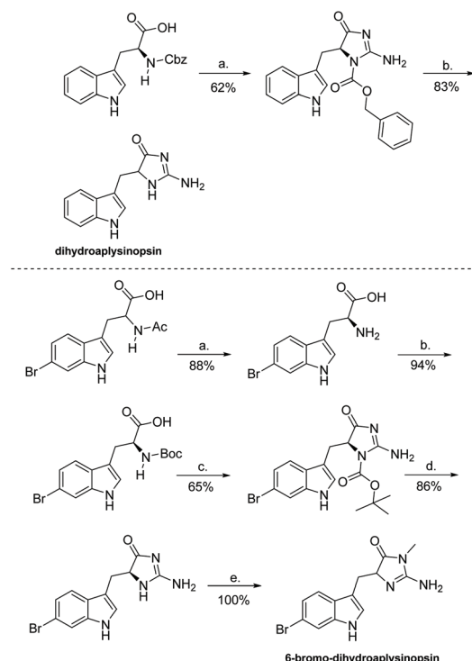
Scheme 31 Total synthesis of dihydroaplysinsin and its 6-bromo derivative. Reagents: (a) 1. THF, DCC, NHS, 0\text{ }^\circ\text{C} , 3 h, 2. \text{NaHNCN} , \text{H}_2\text{O} , rt, 16 h, (b) MeOH, Pd/C, \text{H}_2 , rt, 1 h. Reagents: (a) Borate buffer, \text{CoCl}_2 \cdot 6\text{H}_2\text{O} , pH = 8.5, L-aminoacyclase, 38\text{ }^\circ\text{C} , 48 h, (b) 1,4-dioxane, \text{H}_2\text{O} , KOH, \text{Boc}_2\text{O} , rt, 16 h, (c) 1. THF, DCC, NHS, 2 h 2. \text{NaHNCN} , \text{H}_2\text{O} , rt, 16 h, (d) MeCN, \text{SnCl}_4 , 0\text{ }^\circ\text{C} , under Ar, 45 min, (e) MeCN, EtOH, MeI, rt, 24 h.
