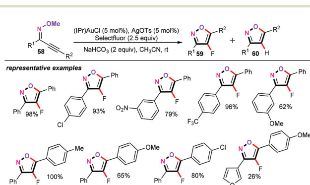
Scheme 27 Gold-catalyzed cascade cyclization/fluorination reaction.
