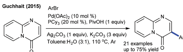
Scheme 17 C3-Arylation of pyrido[1,2- a ]pyrimidin-4-ones.
