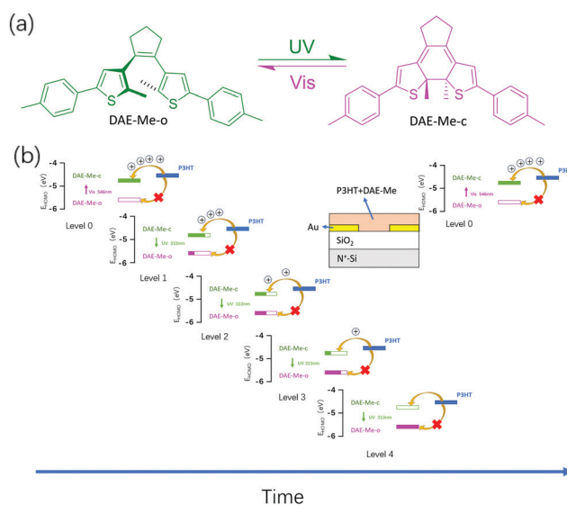
Fig. 17 (a) Chemical structure of the used DAE, in its open and closed form. (b) Middle: Structure illustration of the devices on a \text{SiO}_2 substrate. Schematic diagram of a multi-level storage device. With the increase of the 313 nm ultraviolet light irradiation time, the device gradually changed from level 0 to level 4, and then by 546 nm visible light irradiation, the device returned to level 0.
