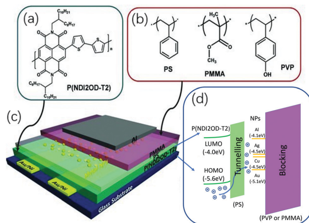
Fig. 2 Molecular structures of (a) the semiconductor P(NDI2OD-T2) and (b) the dielectric PS, PMMA and PVP. (c) Structure of an organic NFGM device based on TG/BC OFET geometry. (d) Schematic illustration of the charge transfer mechanism of the organic NFGM device shown in (c). Reproduced with permission. 35 Copyright 2013, John Wiley and Sons.
