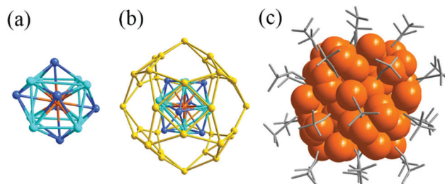
Fig. 16 (a) The \text{Ag}@ \text{Ag}_{14} core; (b) the structure of the \text{Ag}@ \text{Ag}_{14}@ \text{Ag}_{36} shell; and (c) overall structure of \text{Ag}_{51}(\text{BuC}\equiv\text{C})_{32} . Adapted with permission from ref. 36. Copyright 2018, Royal Society of Chemistry.
