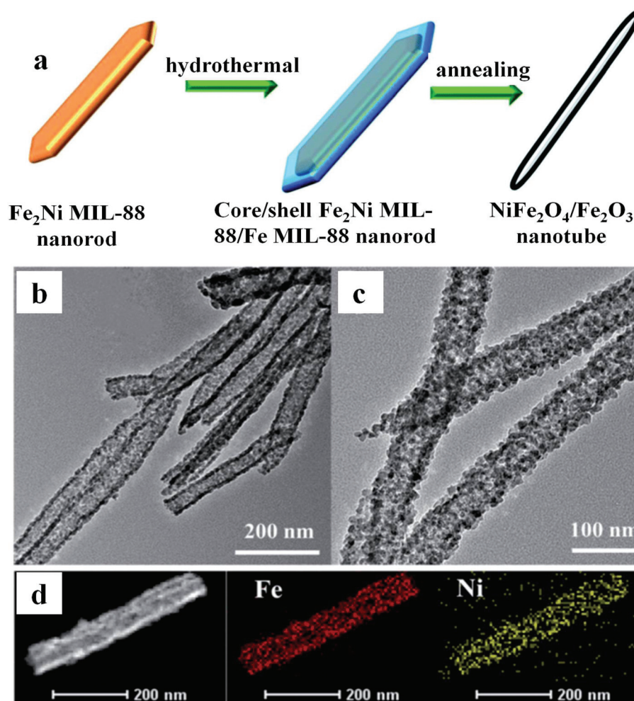
Fig. 3 (a) Preparation process of NiFe 2 O 4 /Fe 2 O 3 nanotubes. (b) and (c) TEM images. (d) HAADF-STEM and elemental mapping. 36
