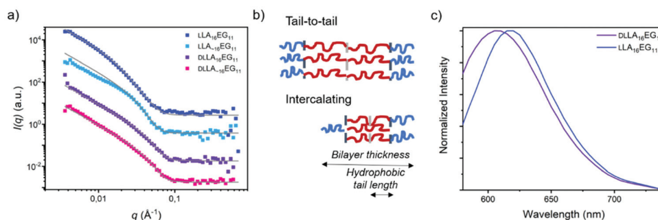
Fig. 5 (a) SANS scattering profiles and corresponding fits in D 2 O, 1 mg mL -1 . Data is shifted vertically for clarity. (b) Schematic representation of possible bilayer structures in solution, LA 16 in red, EG 11 in blue. (c) Normalized emission spectra of the dye NR in self-assembled DLA 16 EG 11 and LLA 16 EG 11 in water.
