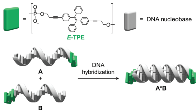
Fig. 1 Sequences of oligomers A–D, chemical structure of the TPE modification and illustration of DNA hybrid A·B.
