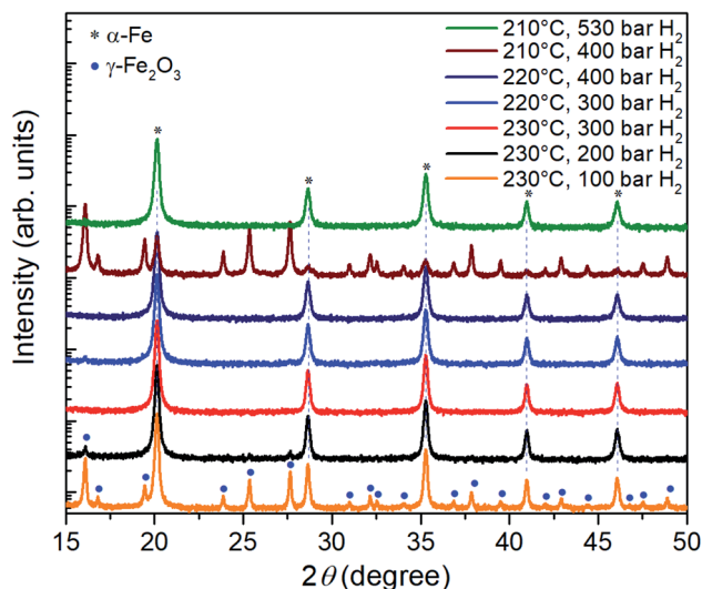
Fig. 3 XRD patterns of the \gamma\text{-Fe}_2\text{O}_3 nanoparticle powders after three-hour reduction at temperatures of 210 °C–230 °C and hydrogen pressures in the range between 100 bar and 530 bar.
