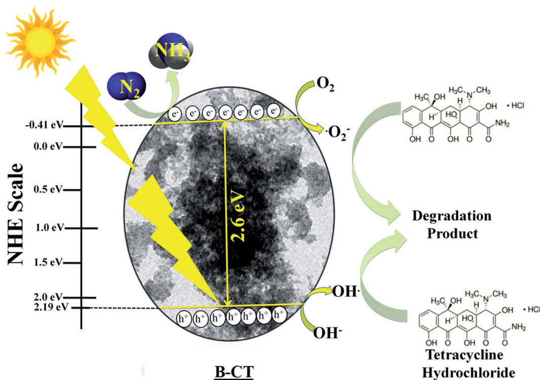
Scheme 3 The mechanism of \text{N}_2 photo-fixation and TCH degradation over B-CT.
