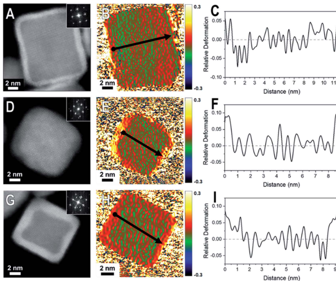
Fig. 3 HAADF-STEM images and corresponding GPA for the thick (5–7 ML) shelled samples (A–C) Pd@Pt, (D–F) Rh@Pd, and (G–I) Rh@Pt nanocrystals. The first column consists of the HAADF-STEM images of the nanocrystal examined by GPA. The second column contains the corresponding GPA color maps which correspond to the in-plane strain ( \epsilon_{xx} ) field (which is the strain in the plane of the crystal face) where the intensity scale shows relative deformation. The third column contains line profiles of the lattice difference determined by GPA with the line profile locations indicated by arrow in the GPA color maps where the start of the line profile begins at the dot and ends at the arrow head.
