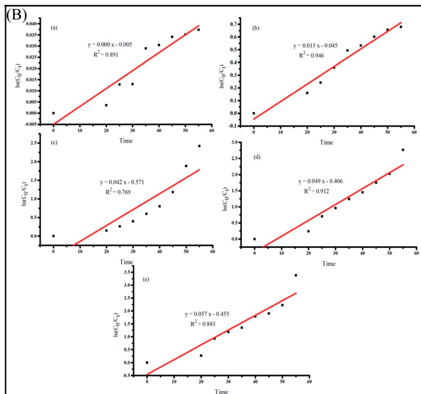
Fig. 6 (A) Percentage photodegradation of PBS dye in aqueous solution over the blank, PC, 1-PSC, 5-PSC, and 7-PSC nanocomposites in the presence and absence of visible light illumination. (B) The rate constants of the curve of the different photocatalysts against PBS dye: (a) blank test, (b) PC, (c) 1-PSC, (d) 5-PSC, and (e) 7-PSC.
