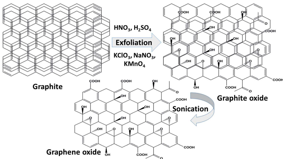
Fig. 5 A schematic representation of the synthesis of GO by chemical methods.
