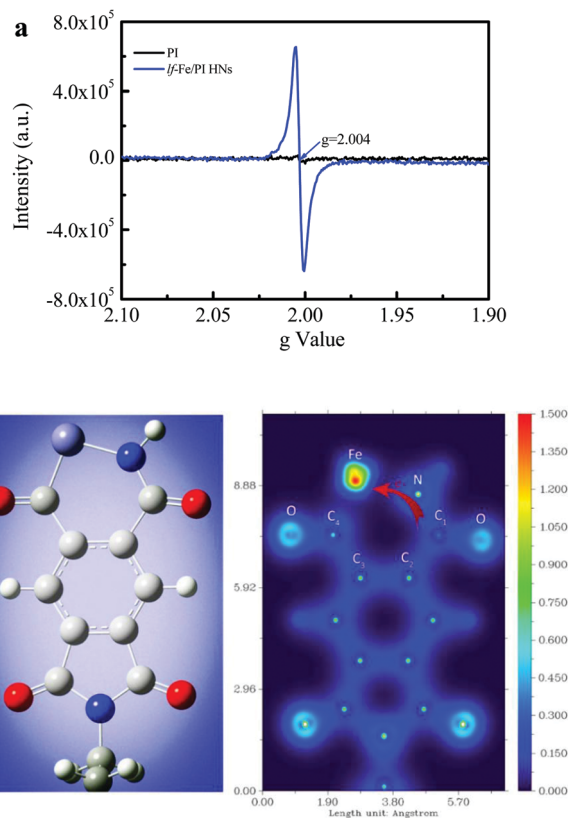
Fig. 4 Non-uniform distribution of surface electrons on If-Fe/PI HNs. (a) EPR spectra of PI and If-Fe/PI HNs. (b) DFT calculations for the optimized structure of If-Fe/PI HNs in one unit (left) and the corresponding two-dimensional valence-electron density color-filled maps of the If-Fe/PI HNs model (right). Purple, red, grey and blue circles denote Fe, O, C and N atoms, respectively. The valence-electron density is given in \text{e} \text{ \AA}^{-3} .
