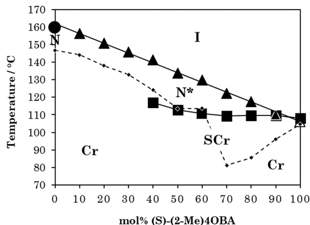
Fig. 2 Phase diagram of binary mixtures of 4OBA and (S)-(2-Me)4OBA, where \blacklozenge represents the melting point, \bullet T_{N_I} , \blacktriangle T_{N^*_{I}} , and \blacksquare T_{SCr/N_I} . An unfilled triangle represents a virtual transition temperature.
