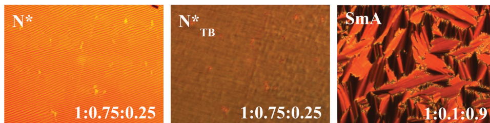
Fig. 3 POM images for 1OB6OS : 4OBA : (S)-(2-Me)4OBA with composition 1 : 0.75 : 0.25 in the N^* and N^*_{TB} phases (left and middle, respectively) in a 3 micron planar aligned cell, and with composition 1 : 0.1 : 0.9 in the SmA phase (right) in untreated glass slides.
