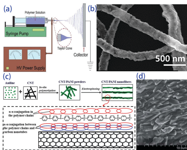
Fig. 4 (a) Scheme of a conventional electrospinning setup, 39 (b) electro-spun hollow PbTe nanofibers, 44 (c) schematic of the formation mechanism and (d) SEM image of CNT/PANI nanofibers. 45
