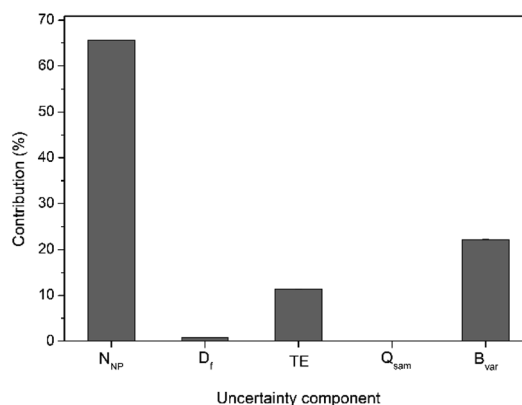
Fig. 3 Typical uncertainty budget for dynamic mass flow method, using 30 \text{ nm} Au NP as an example. N_{\text{NP}} is the number of particles detected in time scan, D_i is sample dilution factor, TE is the transport efficiency, Q_{\text{sam}} is the sample mass flow and B_{\text{var}} is the batch-to-batch variability.
