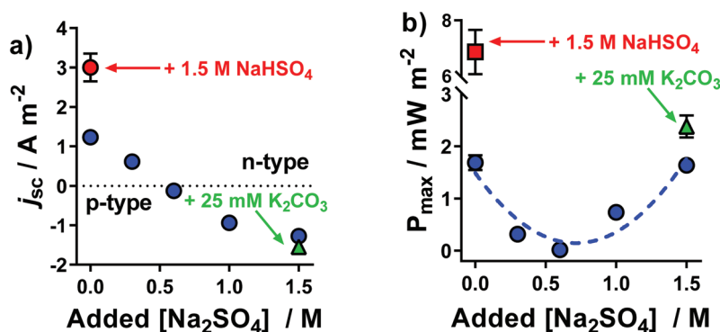
Fig. 2 Plots of the (a) short-circuit current density, j_{\text{SC}} , and (b) maximum power density, P_{\text{max}} , generated by the thermocells as a function of \text{Na}_2\text{SO}_4 concentration; all experimental conditions are the same as Fig. 1. All values are the average of triplicate measurements; error bars represent \pm 1 standard deviation, and no error bars indicate error was equal to or smaller than the size of the data point. The effect of iron sulphate concentration and \text{NaHSO}_4 concentration are shown in Fig. S1.†
