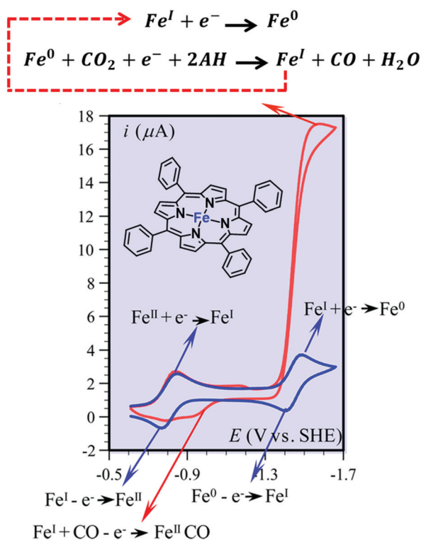
Fig. 2 Cyclic voltammetry of FeTTP ( 1 ) (1 mM) in DMF + 0.1 M n -Bu 4 NPF 6 in the absence (blue) and presence of 0.23 M CO 2 and of 10 mM PhOH (red). Sketch of the electrochemical reactions. Adapted with permission from ref. 86. Copyright 2013 American Chemical Society.
