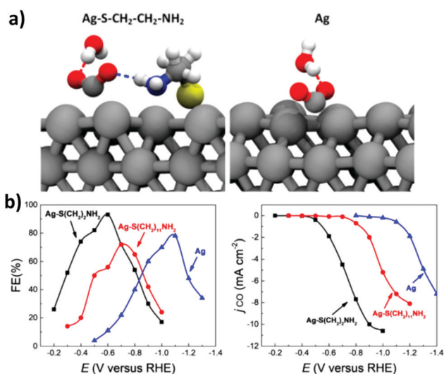
Fig. 31 (a) Chemisorbed \text{CO}_2 on cysteamine-functionalized (left) and cysteamine-free (right) Ag(111) surface. Only the water molecules directly forming hydrogen bond (slashed line) are shown. The colors are: Ag in silver, C in gray, O in red, N in blue, S in yellow, and H in white. (b) Influence of the alkyl chain length on \text{CO}_2 RR in terms of \text{FE}_{\text{CO}} (left) or j_{\text{CO}} (right) vs. potential. Reproduced with permission from ref. 419. Copyright 2018 American Chemical Society.
