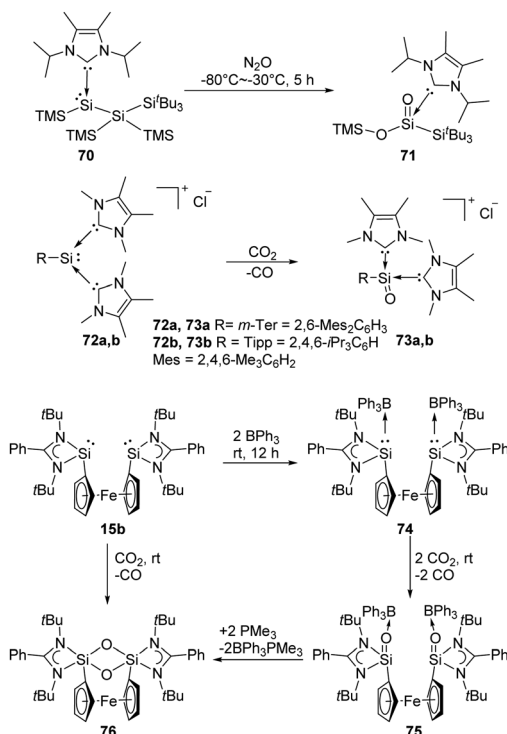
Scheme 27 Activation of \text{N}_2\text{O} and \text{CO}_2 by Lewis acid/base-stabilised \text{Si}^{\text{II}} species 70 , 72a, b , 15b and 74 .
