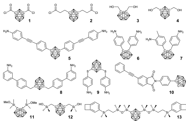
Fig. 2 Borane cluster-containing monomers used in the preparation of the corresponding PIs, epoxy resins, and polysiloxanes.
