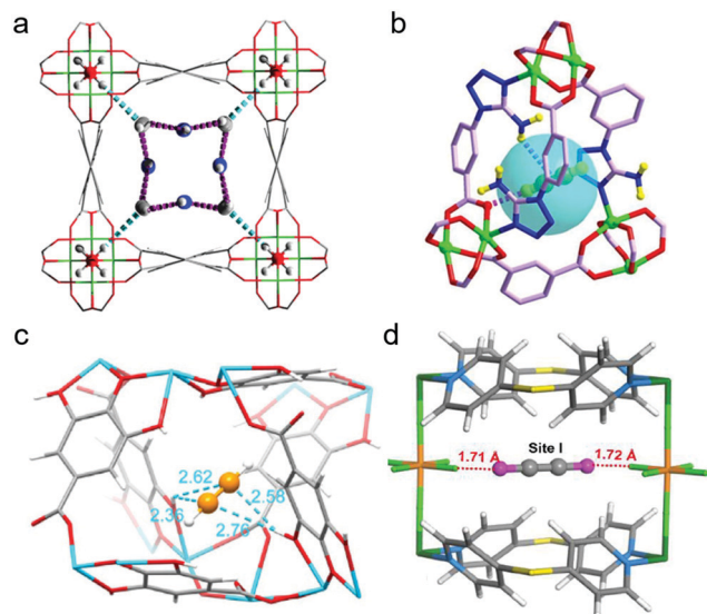
Fig. 11 Preferential C_2H_2 binding sites in C_2H_2/C_2H_4 selective adsorbents: (a) NOTT-300, as determined by DFT-D modelling; 67 (b) UTSA-100a, as determined by DFT-D calculations; 82 (c) Mg-gallate, as determined by NPD experiments; 74 (d) NCU-100a, as determined by Rietveld refinement. 55 (Reprinted with permissions from ref. 67, 82, 55 and 74: copyright 2019, Wiley-VCH Verlag GmbH & Co. KGaA, Weinheim; copyright 2015, Springer Nature; copyright 2020, American Chemical Society; copyright 2014, Springer Nature.)
