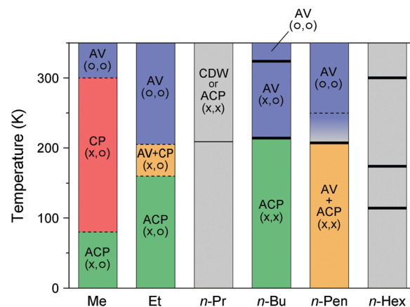
Fig. 10 Temperature dependence of the electronic states of \text{Pt}_2(\text{RCS}_2)_4\text{I} with different alkyl chain ( R ) lengths, where the superlattice structure is not considered. 12,18,31–33,40–43,47–51 Gray areas show the temperature range whose electronic state is unknown, and symbols in parentheses indicate the charge (left) and spin (right) degrees of freedom. Thick and thin vertical lines indicate the first- and higher-order transition temperatures, respectively, observed by heat capacity measurements. 40,48,49,51 For R = \text{Me} , no heat-capacity anomaly was observed at around 300 and 80 K, 47 at which phase transitions occur between the AV and CP states and between the CP and ACP states, respectively. 18 For R = \text{Et} , although numerical data of transition temperatures ( ca. 180 and 230 K) observed by the heat capacity measurements are presented in ref. 12 and 50, the source and full extent of the anomalies are not shown. For R = n\text{-Pen} , no heat-capacity anomaly was observed at around 250 K, 40 at which a conductivity maximum was observed during the resistivity measurements (shown by a dotted line). 41,42
