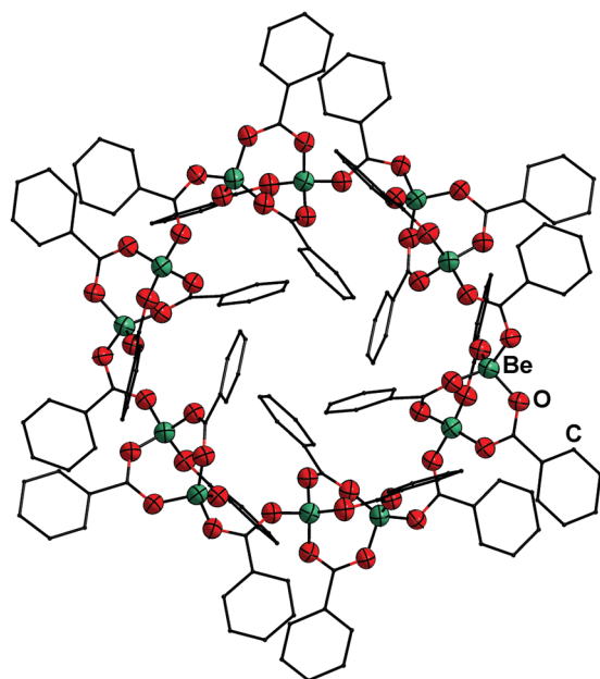
Fig. 3 Molecular structure of [\text{Be}(\text{PhCO}_2)_2]_{12} ( 6 ) in the solid state. Ellipsoids are depicted at 70% probability at 100 K. Carbon atoms are depicted as wire frame and hydrogen atoms are omitted for clarity. 49
