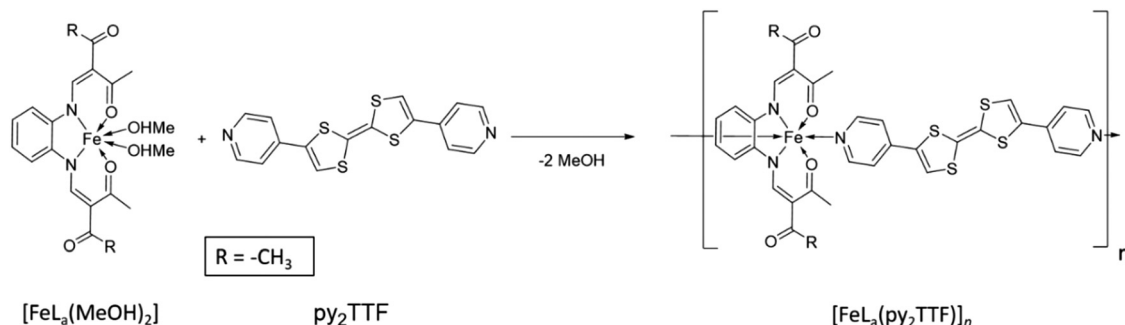
Scheme 1 Synthetic scheme of the iron(II) coordination polymer [\text{FeL}_a(\text{py}_2\text{TTF})]_n ; R = CH 3 (L a )
