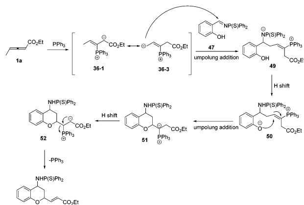
Scheme 15 The possible mechanism for phosphine catalysed (2+4) annulations.
