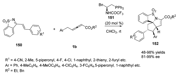
Scheme 48 Bifunctional-phosphine-catalysed sequential annulations of 1-azadiene with \gamma -benzyl allenates.
