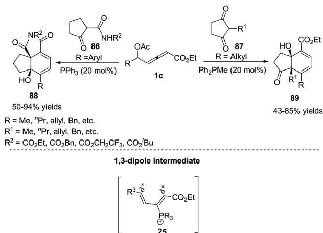
Scheme 28 Phosphine-catalysed (4+2) annulations of \delta -acetoxy allenones and ketones.
