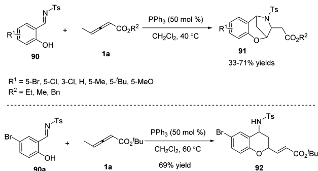
Scheme 29 PPh 3 -Catalysed sequential annulation reactions between salicyl N -tosylimines and allenones.
