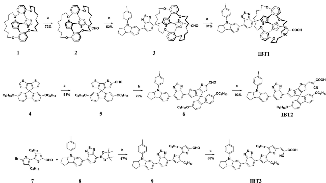
Scheme 1 Synthetic routes of the dyes IBT1–3 . (a) POCl 3 , DMF, and 1,2-dibromoethane, at 80 °C; (b) Pd(PPh 3 ) 4 , Na 2 CO 3 , ethanol, H 2 O, and toluene, at 100 °C; (c) piperidine, cyanoacetic acid, and CHCl 3 , at 75 °C.
