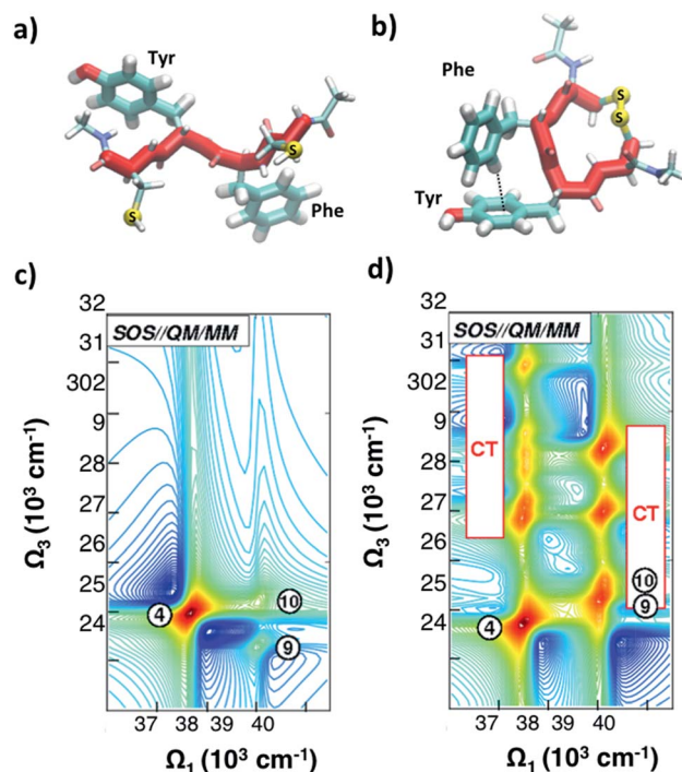
Fig. 8 (a and b) Selected conformations of the unfolded (a) and T-stacked (b) CFYC tetrapeptide. (c and d) Simulated 2DUV spectra obtained with the SOS//QM/MM protocol with a two-color setup and parallel polarizations for: (c) open CFYC; (d) closed CFYC. Reproduced from ref. 110 with permission from the American Chemical Society, copyright 2014.
