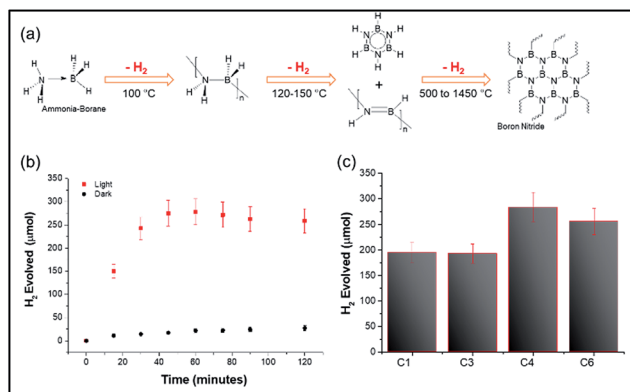
Fig. 5 (a) Schematic of the temperature-dependent decomposition of the ammonia borane complex, ABC (100 \mu\text{mol} ) decomposition by plasmonic (b) DPC-C4 under light and dark conditions and (c) DPC-Cx, using visible to NIR light (400 to 1100 nm wavelength).
