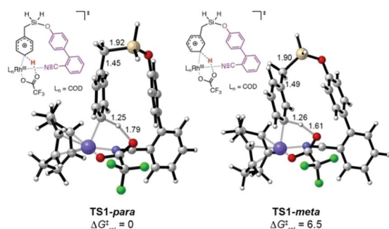
Fig. 1 Transition states for Rh(III)-mediated para -C-H and meta -C-H bond activation, computed with M06/6-311+G(d,p)-SDD//M06/6-31G(d,p)-LANL2DZ in SMD dichloroethane. Distances in Å, \Delta G^\ddagger_{rel} in kcal mol -1 .
