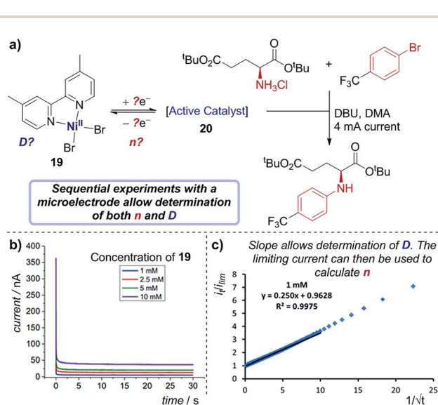
Fig. 20 (a) Determination of both the diffusion coefficient and number of electrons transferred in the reduction of 19 , by the groups of Baran, Minter, Neurock and White. The current response upon application of a potential step is measured (b), and the slope of the plot in (c) allows determination of the diffusion coefficient. Positive current represents reduction. (b and c) Adapted with permission from ref. 39c. Copyright 2019 American Chemical Society.
