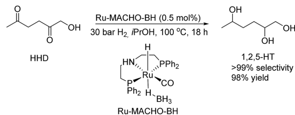
Scheme 13 Homogeneous hydrogenation of HHD.
