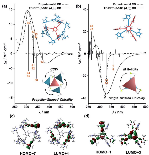
Fig. 8 Dashed lines show experimental CD spectra of (a) (\text{Im}^{\text{R/S}}_3\text{Bz})_4(\text{Zn}^{2+})_3 (corresponding to the red line in Fig. 4) and (b) (\text{ImH}_2)_m(\text{Im}^{\text{S}}_3\text{Bz})_2(\text{Zn}^{2+})_3 (corresponding to the yellow line in Fig. 5). Solid lines show theoretical CD spectra [TD-DFT/B3LYP-6-31G(d,p)] of the C_3 -symmetric ligands in (a) the propeller-shaped arrangement and (b) twisting dimer arrangement. Calculated spectrum in (a) is vertically scaled (scaling factor = 0.85). The numbered excitations correspond to those with high rotatory strength. Two molecular orbitals involved in (c) excitation 43 (17%) in (a) and (d) excitation 14 (47%) in (b). Insets: schematic representation of (a) propeller-shaped chirality and (b) single twisted chirality.
