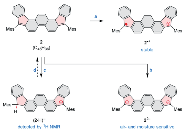
Scheme 3 Redox reactivity of 2 . Reagents and conditions: (a) [\text{p-}\text{C}_6\text{H}_4\text{Br}_3][\text{SbCl}_6] (magic blue). (b) Na metal, \text{THF-}d_8 . (c) Na metal, \text{THF-}d_8 , traces of moisture. (d) Air (partial recovery).
