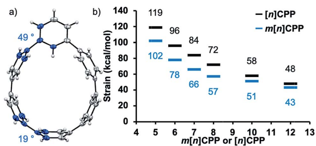
Fig. 2 (a) Molecular structure of m[6] CPP determined by X-ray crystallography (thermal ellipsoids shown at 50% probability). (b) Calculated strain using homodesmotic reactions of [n] CPPs (black) and m[n] CPPs (blue) at B3LYP/6-31G(d,p) level of theory.
