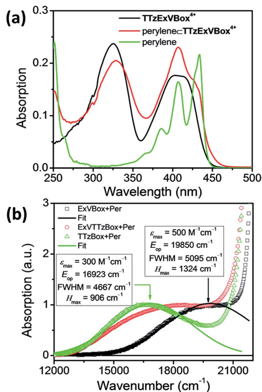
Fig. 3 (a) Steady-state absorption spectra of TTzExVBox 4+ , Per and Per in TTzExVBox 4+ in CH 3 CN. The concentration of Per in the latter two solutions is kept the same. (b) CT bands in Per in ExVBox 4+ , Per in TTzBox 4+ , and Per in TTzExVBox 4+ , and extracted couplings.
