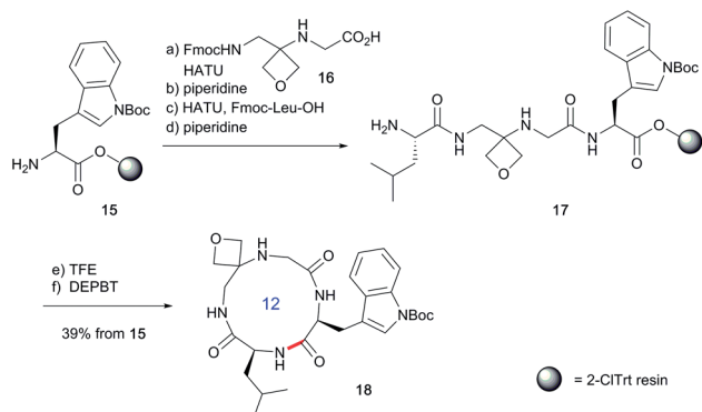
Scheme 4 Synthesis of oxetane modified cyclic peptide 18 by SPPS. Reaction conditions: (a) 16 (2 equiv.), HATU (1.9 equiv.), 1 Pr 2 EtN (4.0 equiv.), DMF, 2–4 h, double coupling; (b) 20% piperidine, DMF, 20 min; (c) Fmoc-Leu-OH (5.0 equiv.), HATU (4.9 equiv.), 1 Pr 2 EtN (10 equiv.), DMF, 1 h; (d) 20% piperidine, DMF, 20 min; (e) TFE/CH 2 Cl 2 (1 : 4), 3 × 1 h; (f) DEPBT (2.0 equiv.), 1 Pr 2 EtN (2.0 equiv.), DMF (0.001 M), 64 h.
