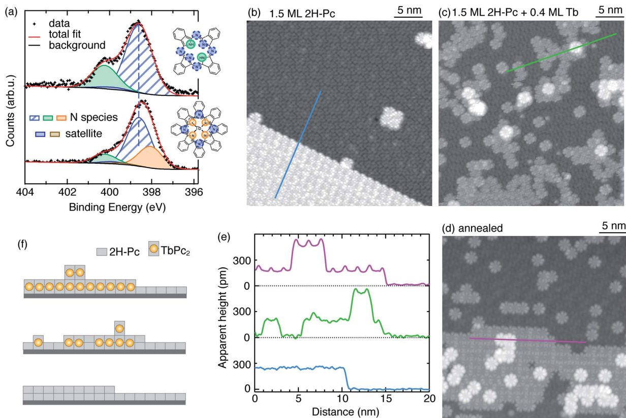
Fig. 2 (a) N 1s XPS spectra and corresponding fit for 1.9 ML pristine 2H-Pc molecules (upper panel) and after deposition of 0.5 ML Tb, yielding 0.5 ML on-surface synthesized \text{TbPc}_2 molecules (lower panel). Schematics of 2H-Pc and \text{TbPc}_2 are shown as insets. For the case of \text{TbPc}_2 , only top layer N atoms are highlighted. STM image of (b) 2H-Pc ( V_t = -2.0 V, I_t = 20 pA, T = 5 K), and (c) \approx 0.4 ML on-surface synthesized \text{TbPc}_2 ( V_t = -2.0 V, I_t = 50 pA, T = 5 K); (d) same as (c) after 15 min of annealing at 500 K ( V_t = -2.0 V, I_t = 50 pA, T = 5 K). (e) Line profiles corresponding to the line-cuts shown in (b), (c) and (d); (f), corresponding models.
