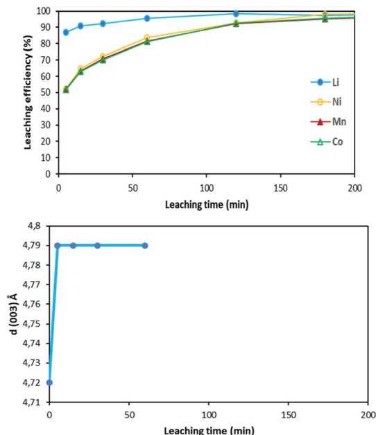
Fig. 13 Comparison between leaching kinetics and d(003) evolution during leaching ( S/L = 80 \text{ g L}^{-1} ; \text{HCl} concentration = 4 \text{ mol L}^{-1} , temperature = 25^\circ\text{C} ).
