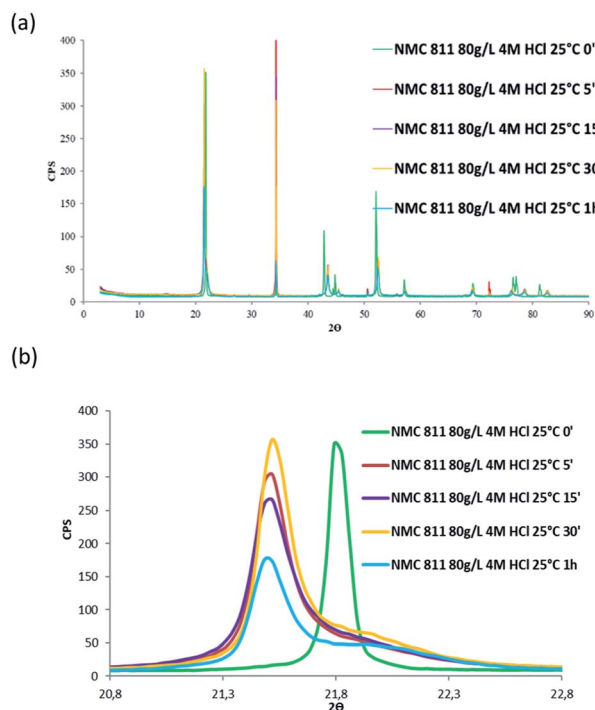
Fig. 12 XRD patterns of (a) NMC 811 and (b) zoom on the peak located between 2\theta = 20.8^\circ and 2\theta = 22.8^\circ during acid leaching ( S/L = 80 \text{ g L}^{-1} ; \text{HCl} concentration = 4 \text{ mol L}^{-1} , temperature = 25^\circ \text{C} ).
