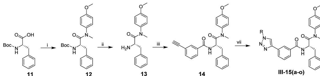
Scheme 3 Reagents and conditions used to synthesize III-15(a–o) . (i) 4-methoxy- N -methylaniline, PyBop, DIEA, \text{CH}_2\text{Cl}_2 , r.t., 8–10 h; (ii): \text{CF}_3\text{COOH} ; \text{CH}_2\text{Cl}_2 , r.t., 5–6 h; (iii) 3-ethynylbenzoic acid, HATU, DIEA, \text{CH}_2\text{Cl}_2 , r.t., 10 h; (vii): azide substituents; \text{CuSO}_4 \cdot 5\text{H}_2\text{O} , VcNa, \text{THF}/\text{H}_2\text{O} ( v : v = 1 : 1 ), 30–60 °C, 4–6 h.
