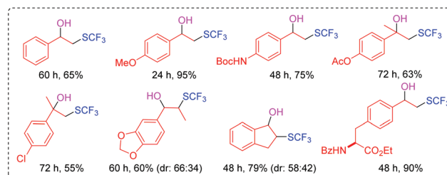
Scheme 7 Trifluoromethylthiolation of aromatic alkenes.
