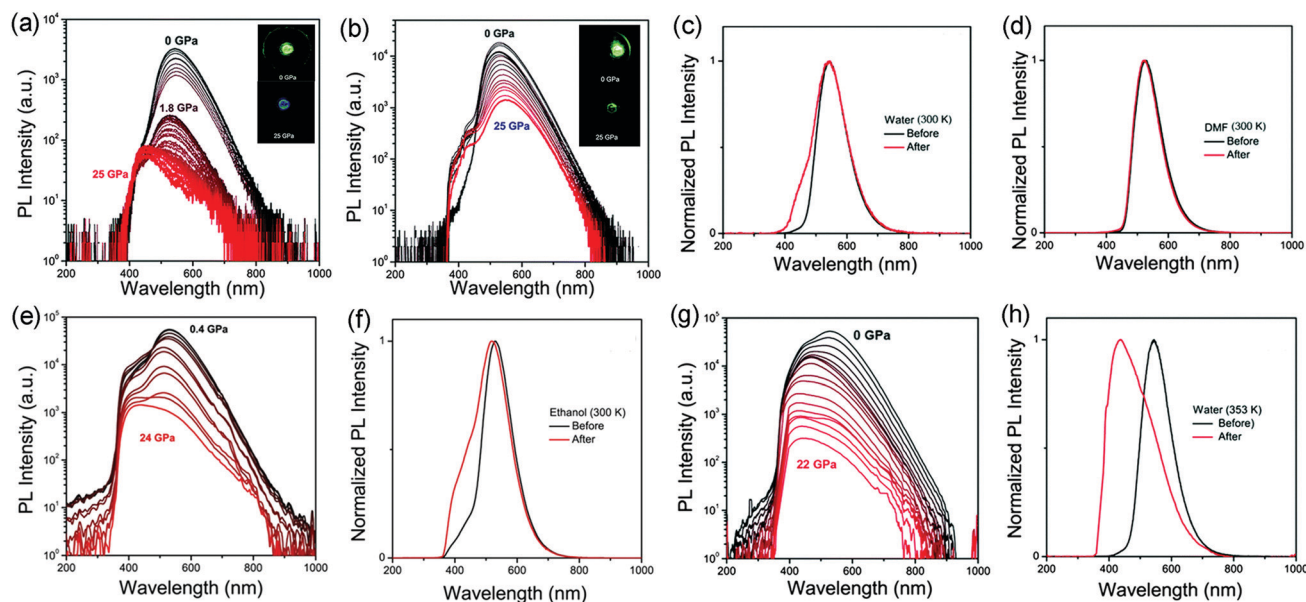
Fig. 3 PL spectral evolution and images of CDs in (a) water and (b) DMF with the increasing pressure from atmospheric pressure to 25 GPa. PL spectra before (black) and after (red) high pressure experiments with (c) water and (d) DMF as PTMs at room temperature (300 K). (e) PL spectral evolution and photographs of CDs in ethanol with increasing pressure from 0.4 GPa to 24 GPa. (f) PL spectral evolution of CDs in ethanol under high pressure at room temperature (300 K). (g) PL spectral evolution of CDs in water at a high temperature of 353 K. (h) PL spectra before (black) and after (red) high pressure experiments with water as the PTM at high temperature (353 K). Reproduced from ref. 39 with permission from The Royal Society of Chemistry.
