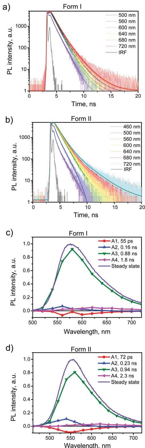
Fig. 5 PL kinetics of BFMPT polymorphs: PL time profiles recorded using form I (a) and form II (b) over the whole emission band after the excitation at 375 nm; the solid lines represent 4-exponential fits convoluted with the instrument response function (IRF); decay associated spectra obtained from 4 exponential fits of fluorescence time profiles for form I (c) and form II (d) in comparison with steady-state spectra recorded using 375 nm laser excitation.
