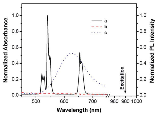
Fig. 2 UCL spectrum of DSPPC-coated NaYF 4 :20%Yb,2%Er (DSPPC-UCNP) under excitation from a 980 nm laser (a), and UV-vis spectra of the protein apo-azurin in the absence (b) and presence of Cu 2+ (c).
