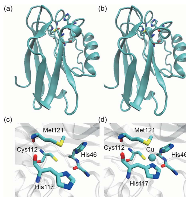
Fig. 3 (a and b) Three-dimensional illustration showing the structure of (a) apo-azurin with a \beta barrel structure without Cu 2+ and (b) azurin with Cu 2+ ; the Cu 2+ -binding domain (c) without and (d) with Cu 2+ coordination.
